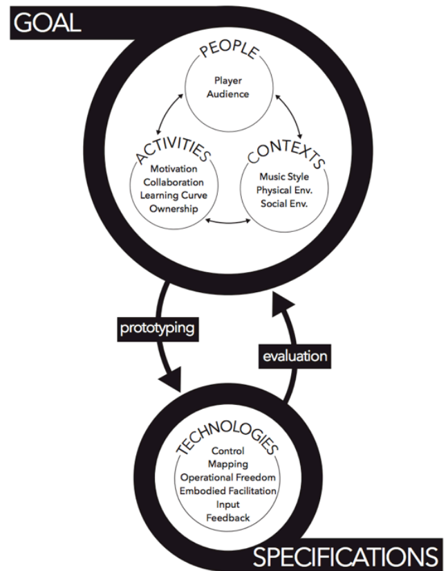
Figure 2 - MINUET framework [17]
