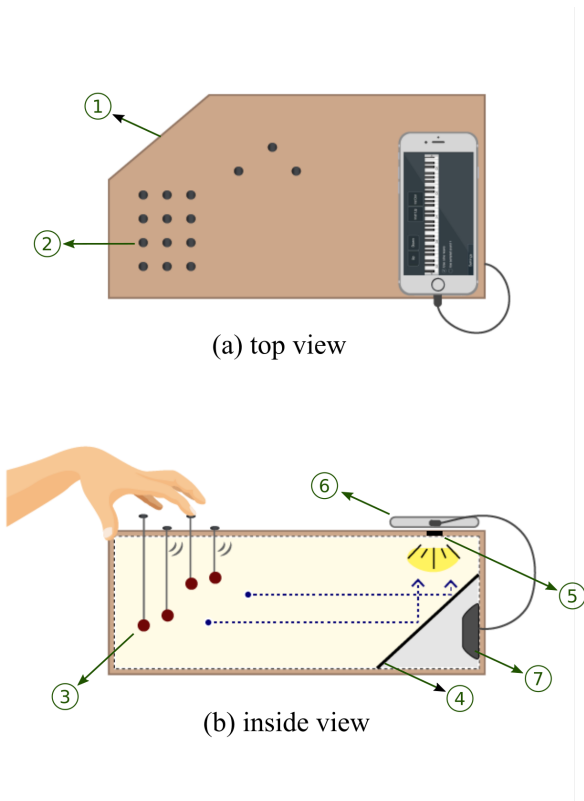
Figure 2: Schematic of the optical push-button system.
