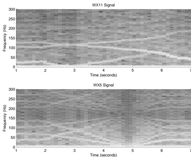
Figure 5: MIDI pressure signals from WX11 and WX5 wind controllers during upward hum.
