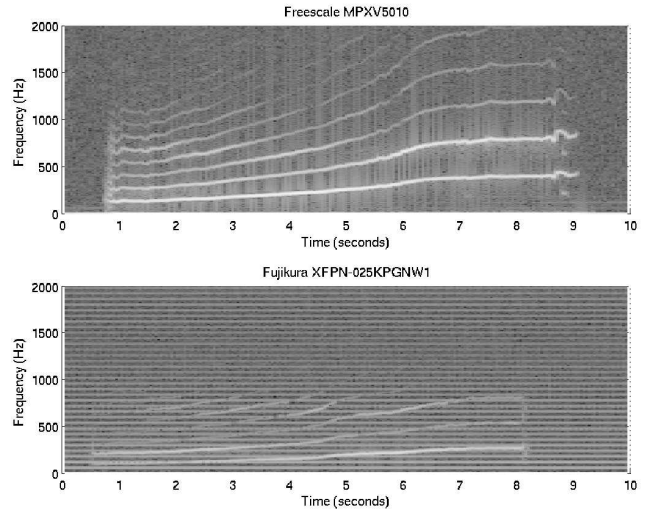
Figure 4: Pressure spectrograms as measured with Freescale and Fujikura sensors during upward hum.
