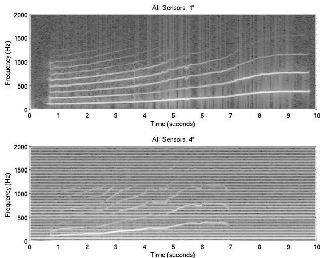
Figure 3: Pressure spectrograms as measured with All Sensors 1" and 4" devices during upward hum.
