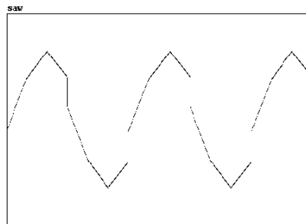
Figure 4. Discontinuities and Reflections in Pd
