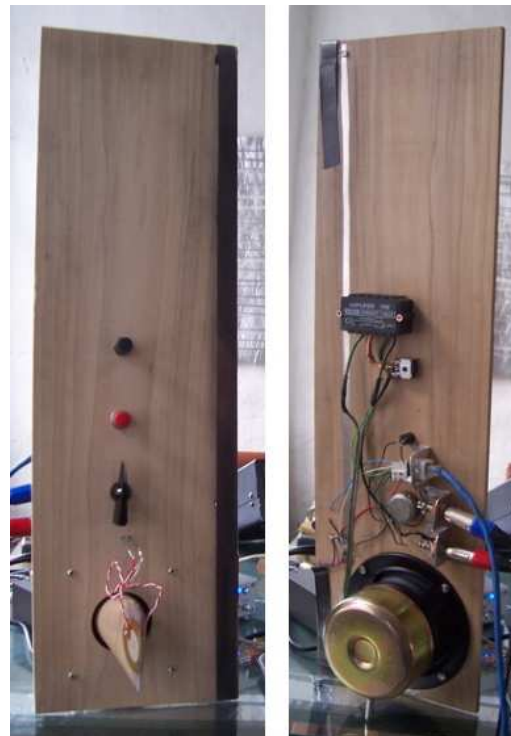
Figure 4: Cellomobo front (left) and back (right)
