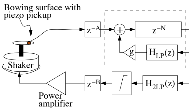
Figure 5: The Cellomobo block diagram
