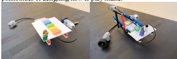
Figure 1. Examples of instruments. Left: The instrument is played by pointing a color sensor towards the colored bricks. Right: The instrument is played by moving ones hands in front of two distance sensors.
