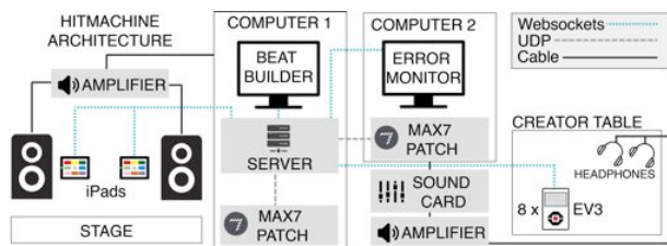
Figure 5. Central components and architecture of Hitmachine.
