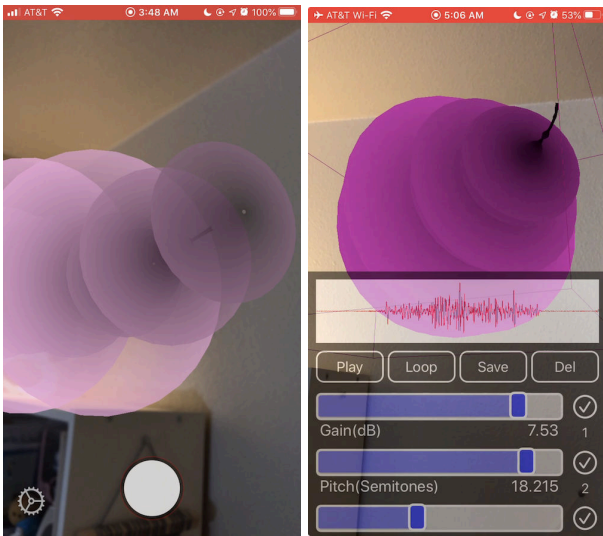
Figure 2: Waveform visualization (left) and sound control GUI (right).
