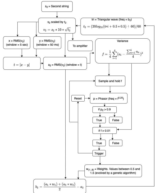
Figure 5: Amplitude sync
