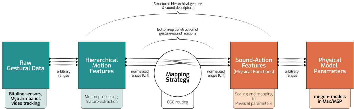
Figure 1: Hierarchical multilayered mapping model from gesture to physically-based sound.
