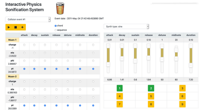
Figure 4: IPSOS Front-End Web Interface.
